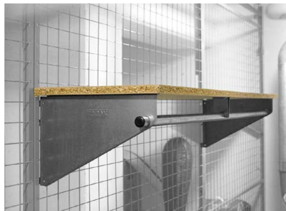
Flexible chipboard shelf with brackets.
